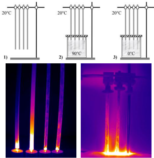
Picture 2. Design of the “heat conduction” experiment and possible solutions
